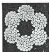
8. Internal corrosion prominent while external surface shows little evidence of deterioration. Complete lack of strand gap suggests internal degradation.
