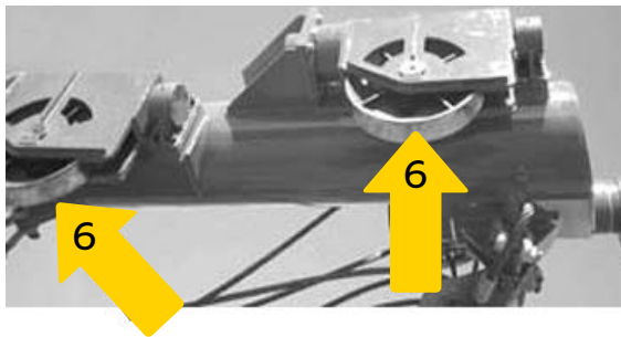
6. Check the condition of the sheave, looking for cracks, dents, rope marks, and the correct rope groove diameter for the rope ( <\pm 5\% of each other).
